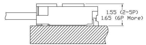
MATING VIEW
