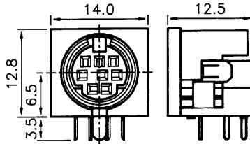
STANDARD TYPE (MDC-023~MDC-028)
