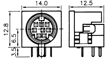
QUICK LOCK TYPE (MDC-053~MDC-058)
