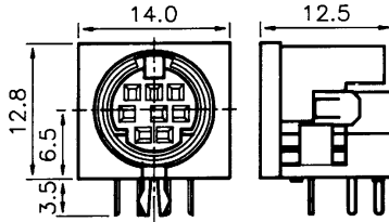
SNAP IN FIT TERMINAL TYPE (MDC-083~MDC-088)
