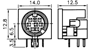
QUICK LOCK & SNAP IN FIT TERMINAL TYPE (MDC-133~MDC-138)
