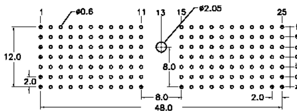
P.C. Board Layout (Top View)
