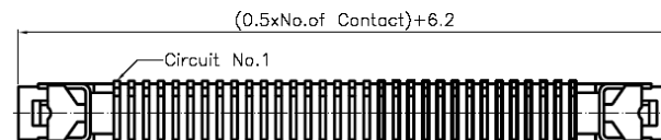
FPC/FFC Dimension Thickness 0.30mm
