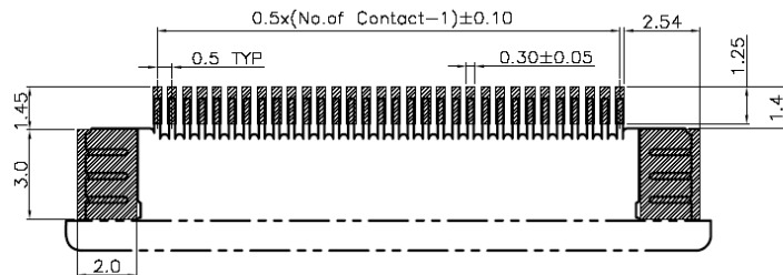
Solder Nail close Type Recommend PCB Layout
