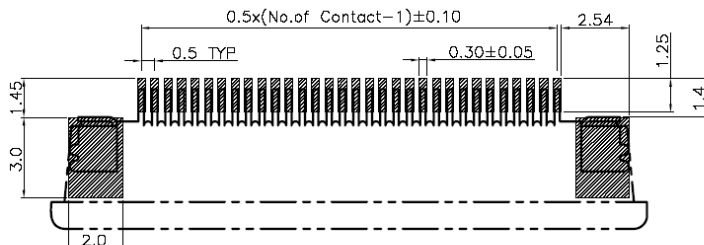
Solder Nail open Type Recommend PCB Layout
