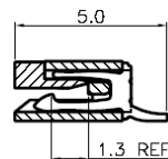
FPC/FFC Dimension Thickness 0.30mm
