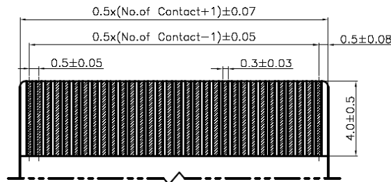
FPC/FFC Dimension Thickness 0.30mm
