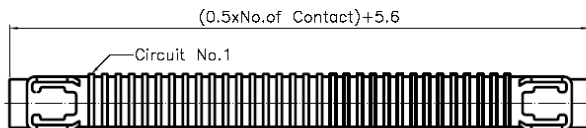
Solder Nail open Type Recommend PCB Layout
