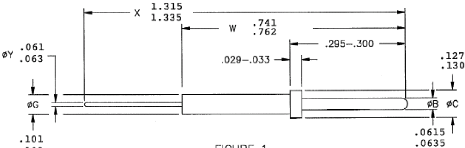
FIGURE 1 PIN CONTACT
