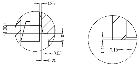
DETAIL C SCALE:4:1
