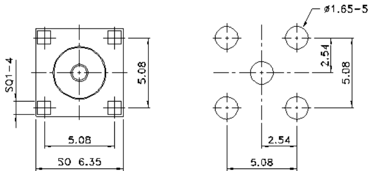
PCB MOUNTING HOLES (印刷电路板架設孔)
