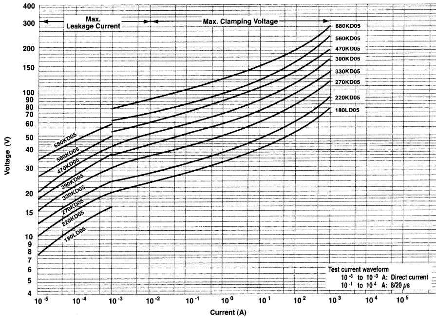
V-I Curve (180L to 680K)
