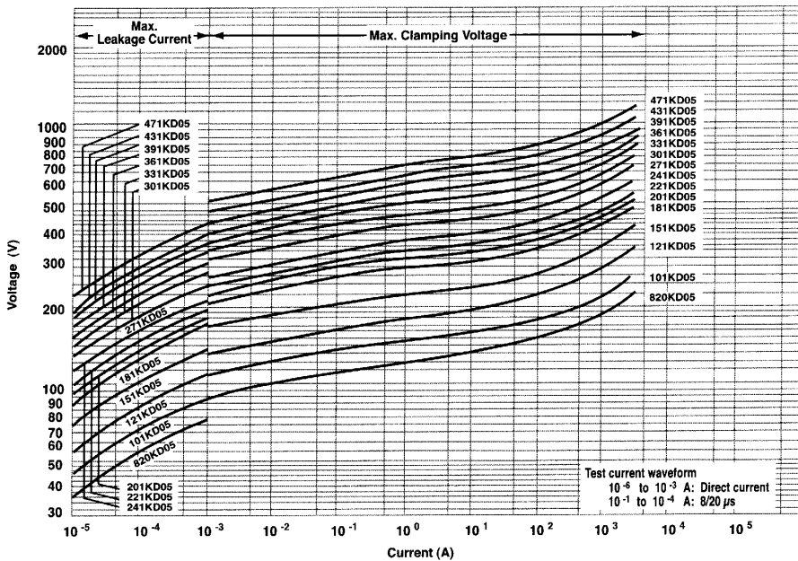
V-I Curve (820K to 471K)
