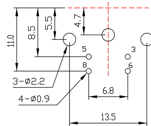
P.C.B LAYOUT ( \pm 0.1 ) (BOTTOM VIEW)
