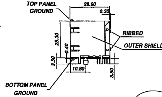
PANEL GROUND MODE
