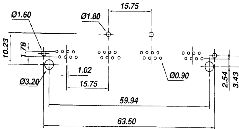
PCB LAYOUT
