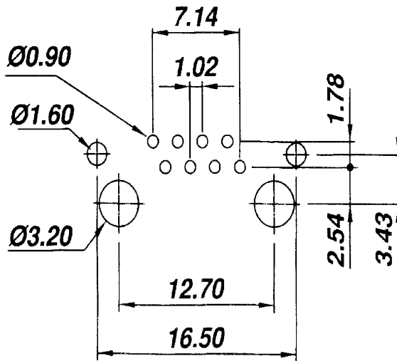
PCB LAYOUT
