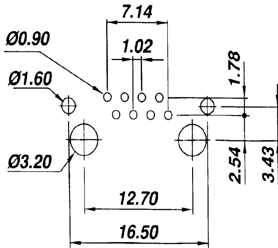
PCB LAYOUT
