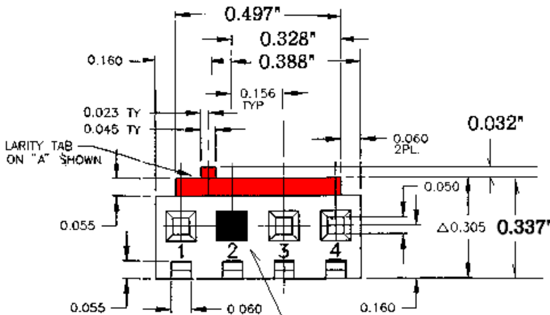
Pin 2 blocked Mating Side
