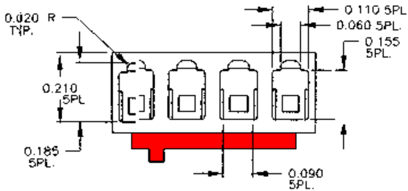
Wire entry side
