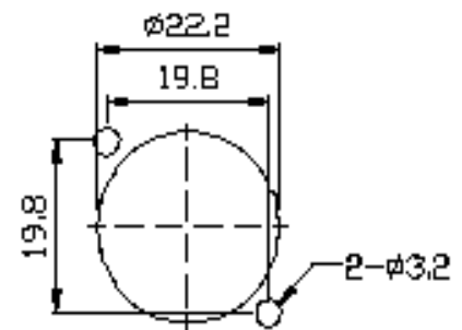
PANEL CUT OUT(±0.05) (FRONT SIDE)
