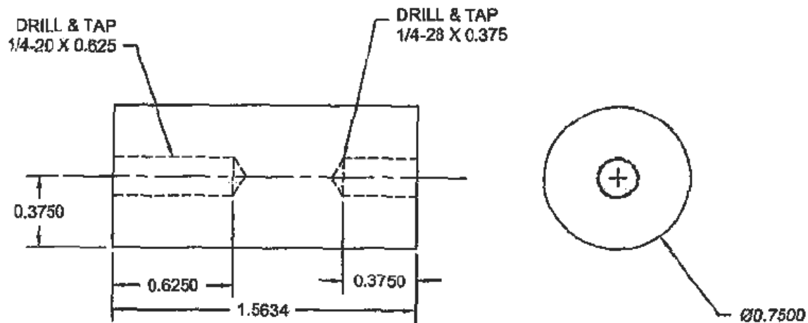
DETAIL ITEM 36
