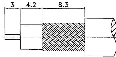
RECOMMENDED CABLE STRIPPING DIM'S (建議剝線尺寸)
