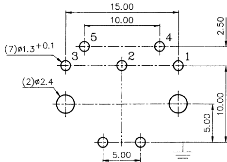
MOUNTING HOLE (TOP VIEW)
