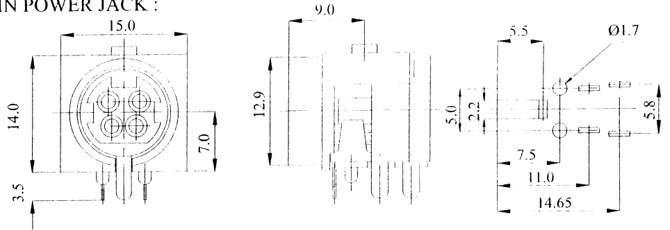
4PIN POWER JACK WITH SHIELD :
