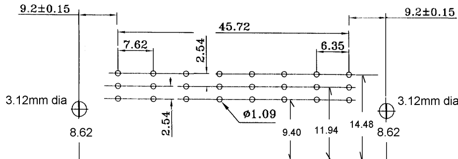
Rear Flange Ref. PCB LAYOUT
